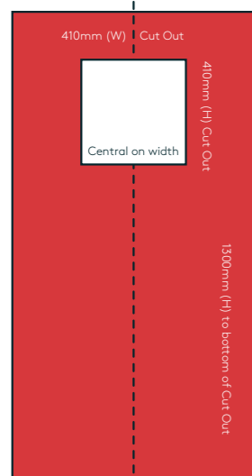
Square VP Cut Out Central Across Leaf Width
