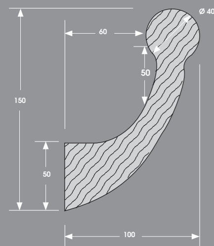
HBN 00-04 ICRW-04-DM Anti-Ligature HBN 00-04 Handrail
