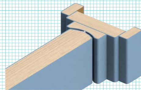
Post-Formed Door & Frame
