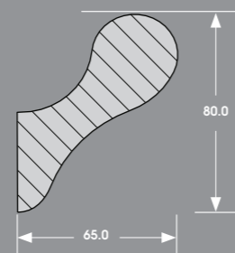
ICRW-04 Ant-Ligature Handrail (ability to ascend upstairs).
