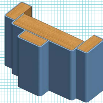
Standard Post-Formed Frame
