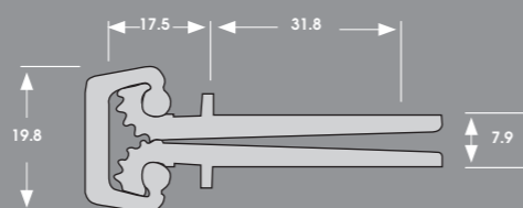
Standard SECURA™ Hinge
